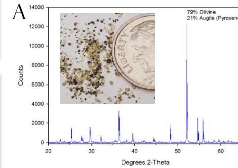
(A) Diffractogram of Hawaiian green sand
