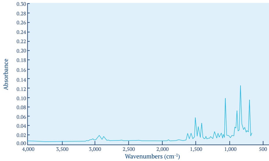
FIGURE 8: FTIR Absorbance Spectrum of Parylene D
