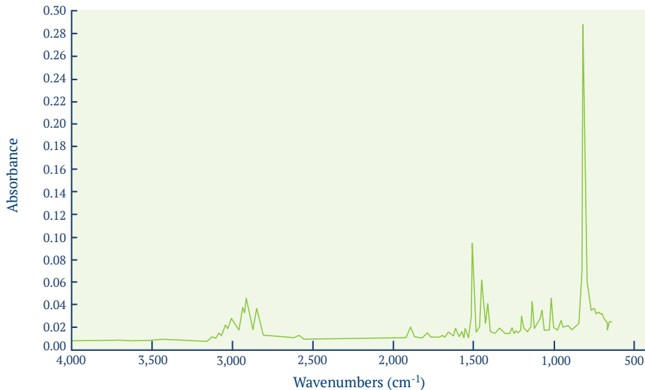
FIGURE 5: FTIR Absorbance Spectrum of Parylene N
