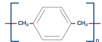
FIGURE 1: Parylenes N, C, D and Parylene HT Chemical Structures
