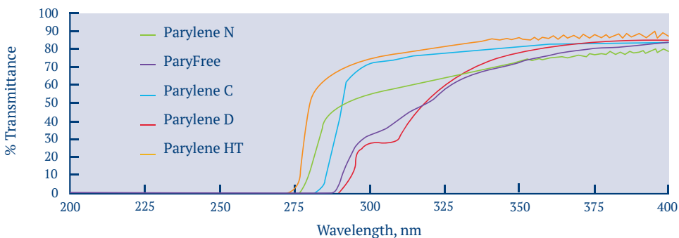
FIGURE 4: Ultraviolet Spectra of Parylenes N, C, D, HT and ParyFree
