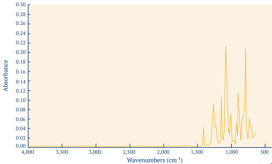
FIGURE 9: FTIR Absorbance Spectrum of Parylene HT
